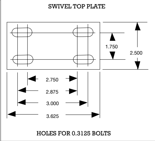
NO. 16 TOP PLATE (STANDARD ON 60 SERIES)
